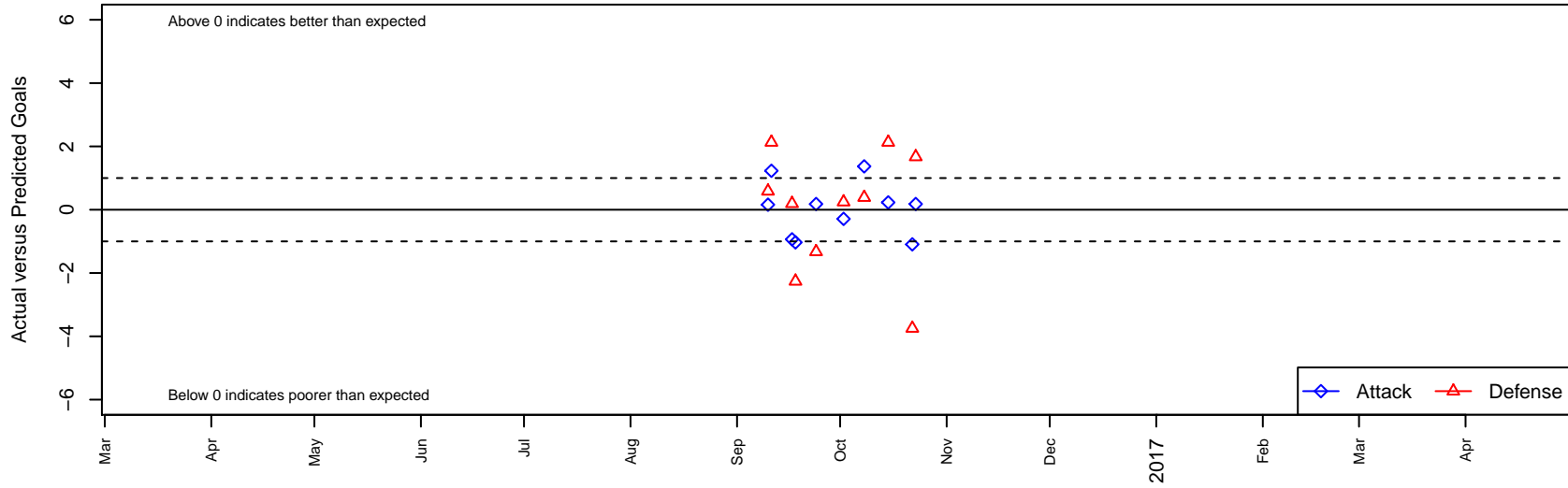
Ashland SC Crossfire G03 Dots are actual minus expected GF (blue circles) and GA (red triangles). Blue line is smoothed change in attack strength. Red is smoothed change in defense strength.
